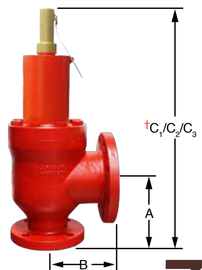
3" FLANGED VALVE
