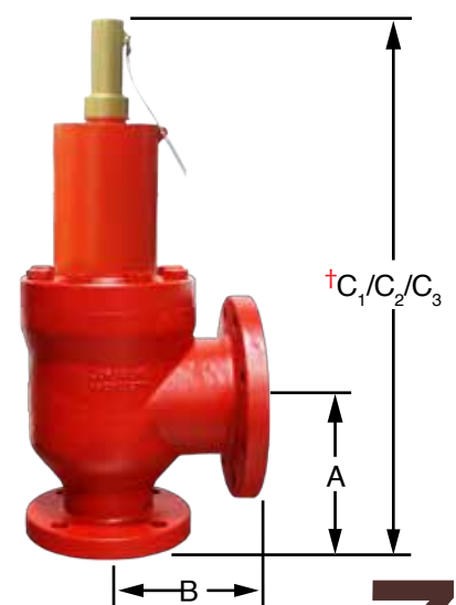
3" FLANGED VALVE
