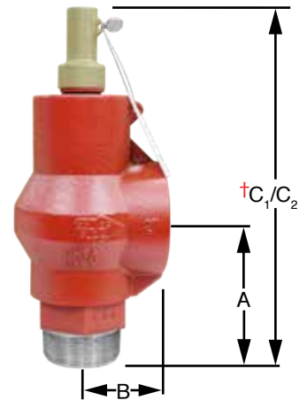
2" THREADED VALVE
