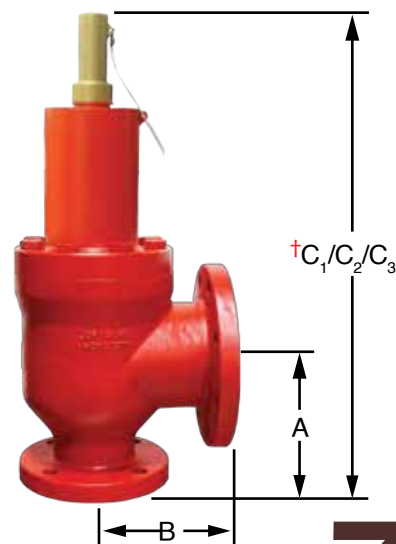
3" FLANGED VALVE
