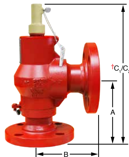
2" FLANGED VALVE
