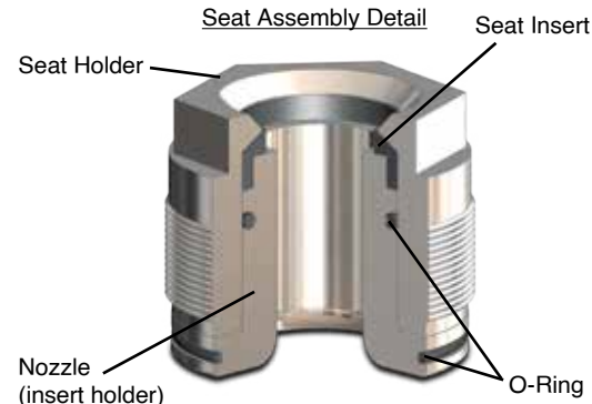
Seat Assembly Detail
