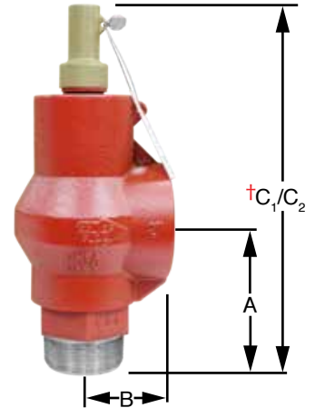
2" THREADED VALVE
