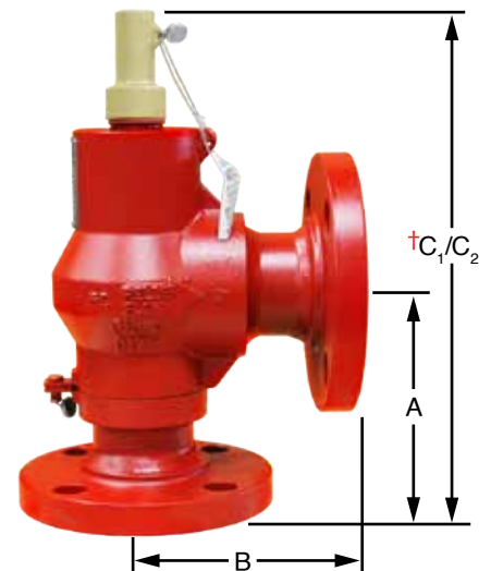
2" FLANGED VALVE
